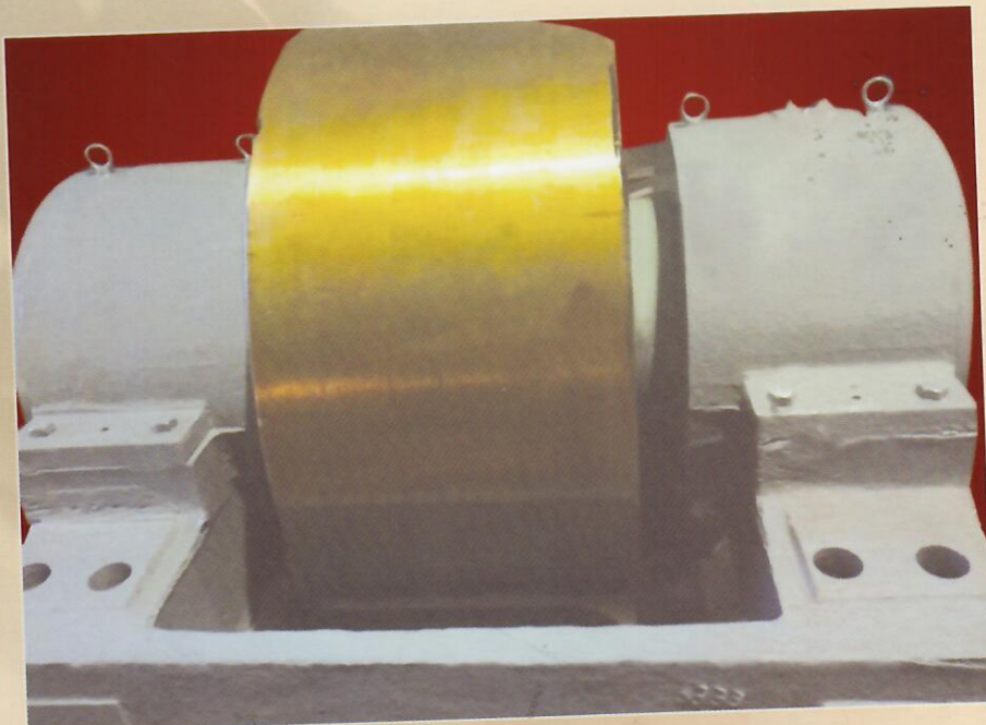
Support Roller Complet Assembly upto 500 T.P.D. for Kiln and Cooler
