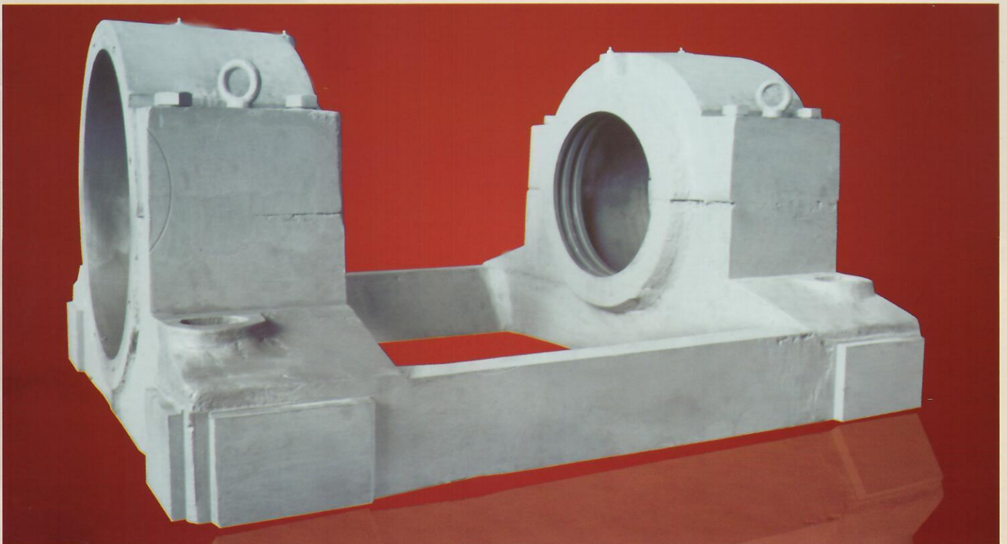
Bearing Housing For Kiln Support Roller upto 500 T.P.D
